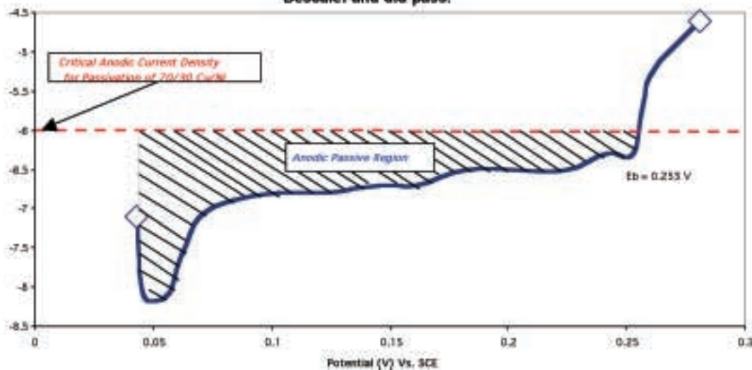
Anodic Polarization Behavior of Experimental Sample #3 After Exposure to Natural Seawater for a minimum of 21 Days Followed by 6 Hr Immersion in Dynamic Descaler, Sample was tested on day one following exposure to Dynamic Descaler and did pass.
